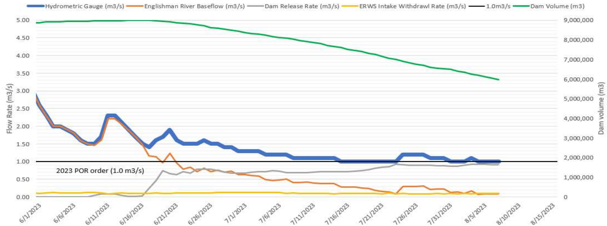
2023 Englishman River & Arrowsmith Dam Flows & Levels
