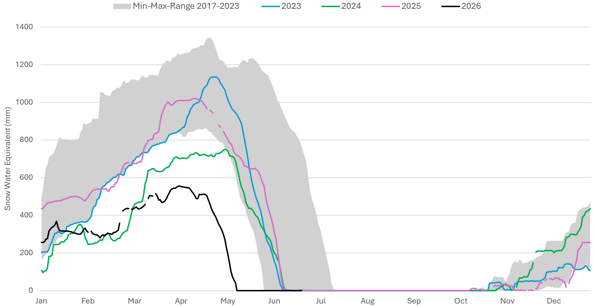
Snow Water Equivalent – Station 3B26P
