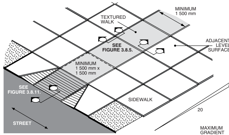
FIGURE 3.8.6. – Walks
