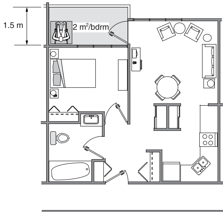
FIGURE 3.8.63. – Residential Balcony
